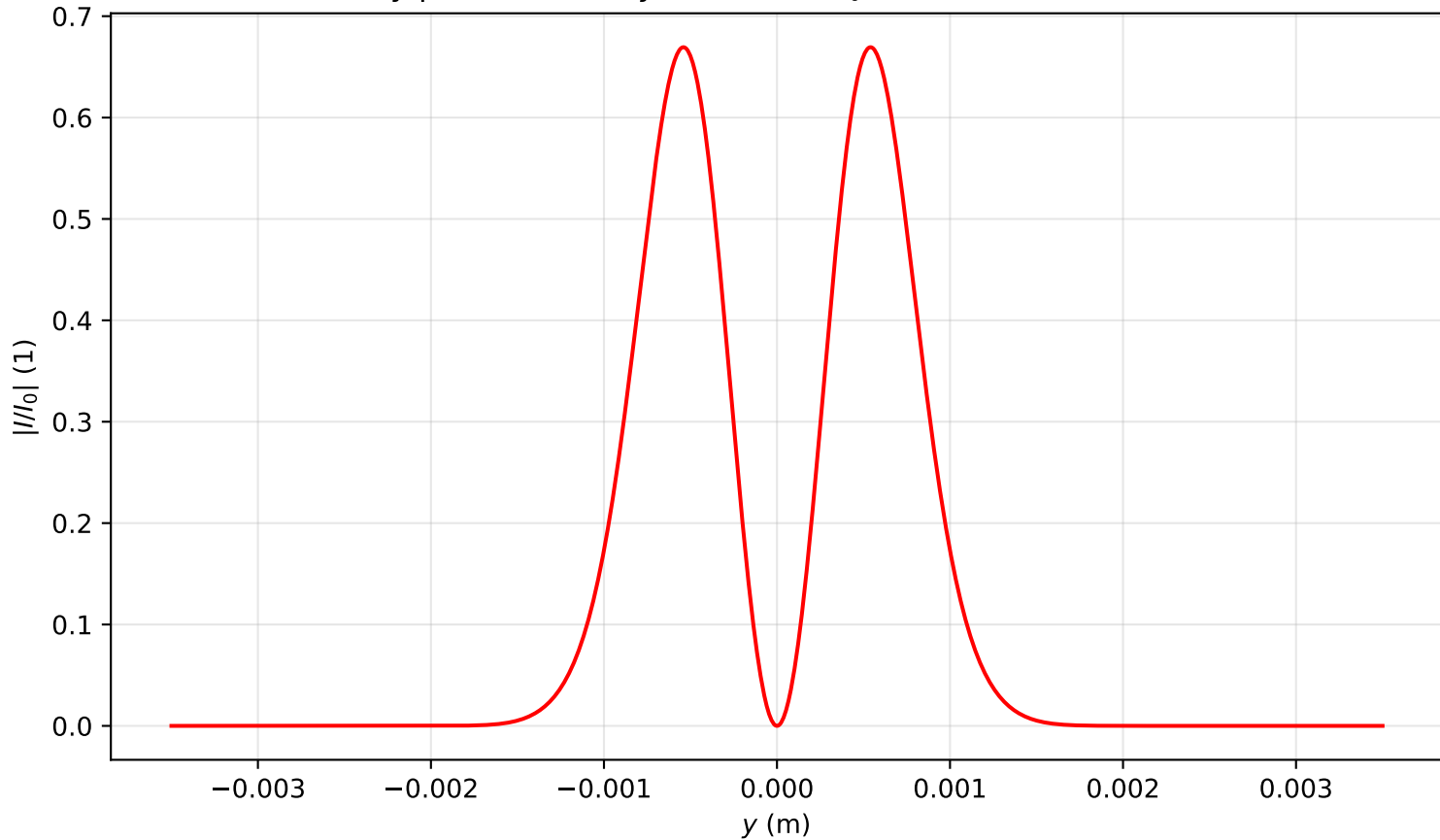
Intensity profile I(x=0, y, z=0.796)/I_0 , P_{in}=0.5P_{cr} , artificial time
